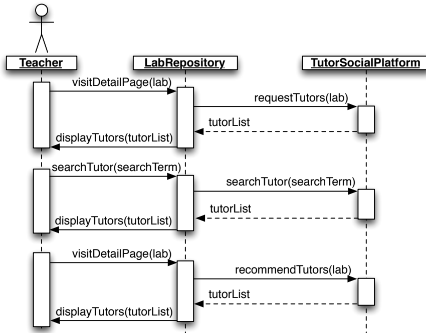
Figure 13.: A sequence diagram that models the listing, searching and recommending of tutors in the bartering platform.
